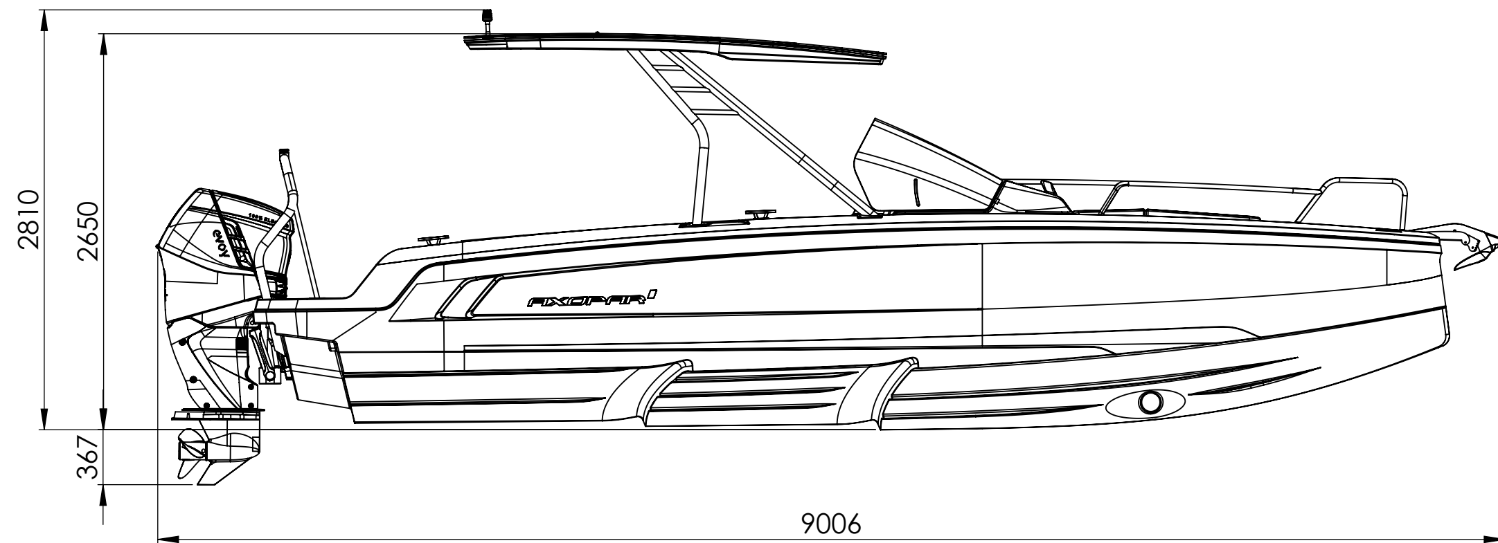
SIDE VIEW
