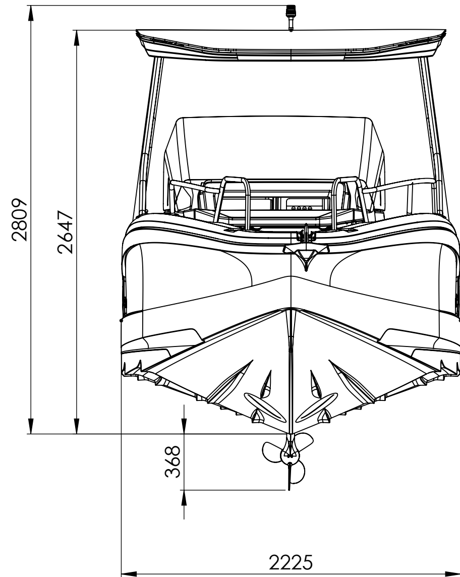
FRONT VIEW
