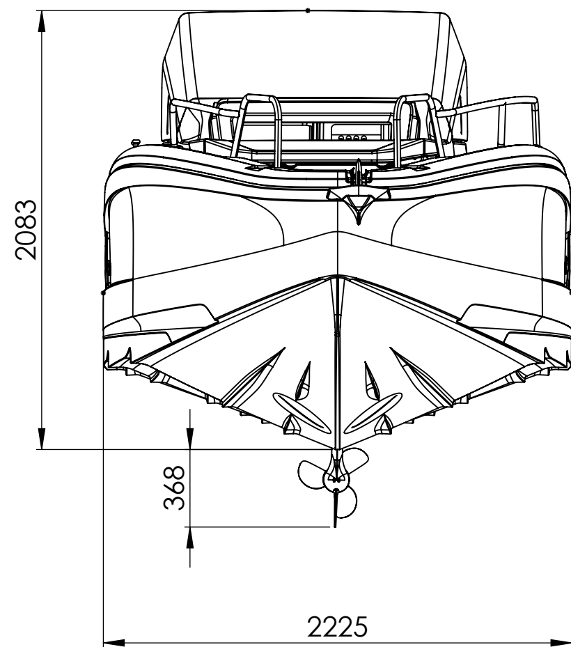
FRONT VIEW
