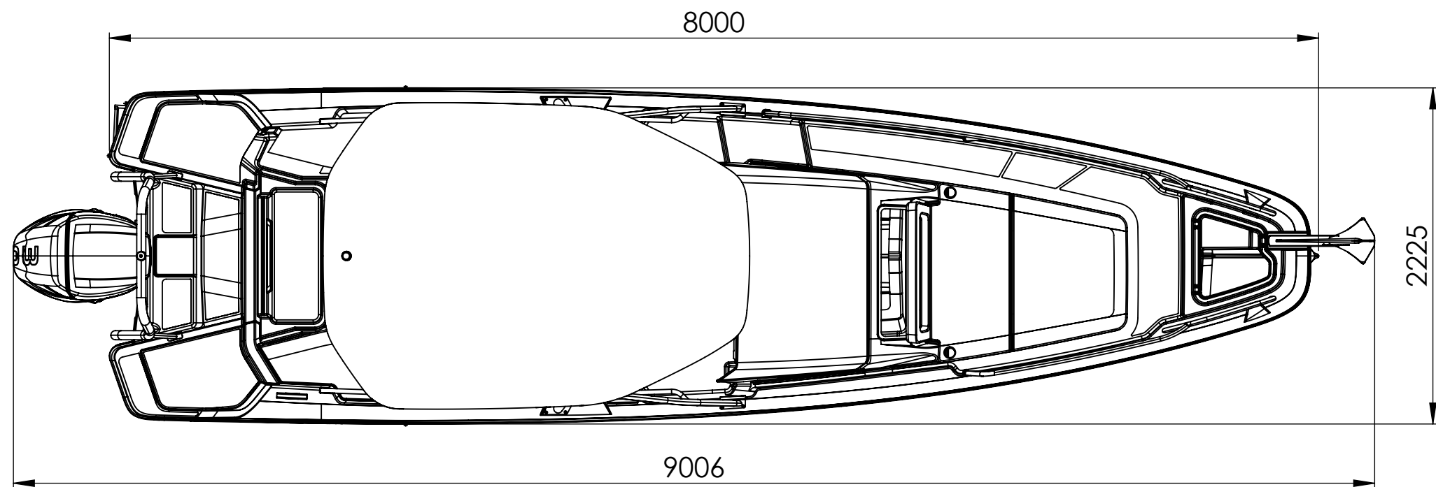
TOP VIEW
